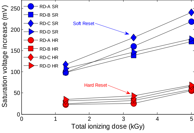
Fig. 2 Saturation voltage increase with irradiation for two reset modes: soft reset (SR) with V_{RST} = 3.3V and hard reset (HR) with V_{RST}
