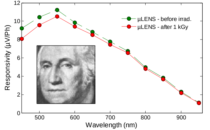
Fig. 5. Responsivity of the image sensor with microlenses prior to and after 1 kGy irradiation and image captured with the irradiated device.
