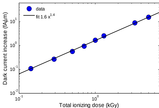
Fig. 7. Radiation induced dark current linear density increase as a function of total ionizing dose at 23°C. Junction perimeter = 35μm.
